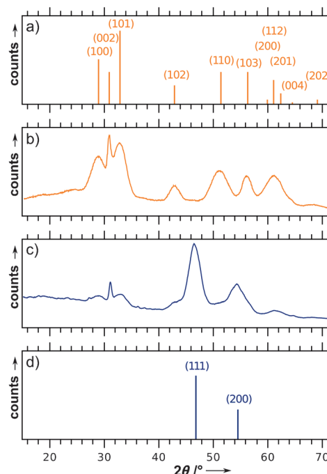
Figure 2. X-ray diffraction patterns of b) CdS nanorods and c) faceted Pt-tipped CdSe@CdS nanorods. For comparison, reference diffractograms are given for a) CdS and d) Pt.
